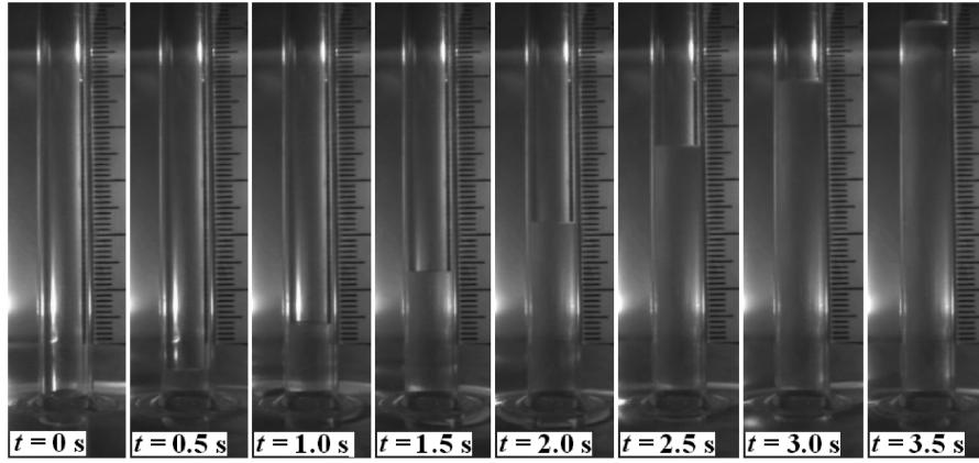
Fig. 2 Selected frames of capillary-driven flow of Eth/H 2 O 30/70(%vol.) into a tube from the experiment video under microgravity condition in the drop tower Beijing. The internal diameter d = 6 mm and the initial liquid height h_0 = 10 mm.
